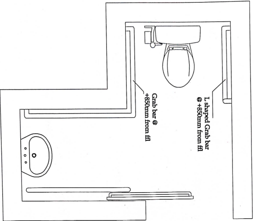
Divyangjan Toilet @ ground floor Layout
